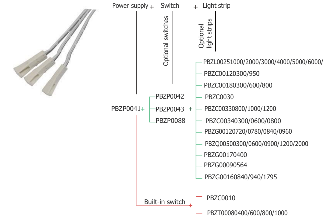
Hardware match figure 1 (power supply & switch & light strip)
