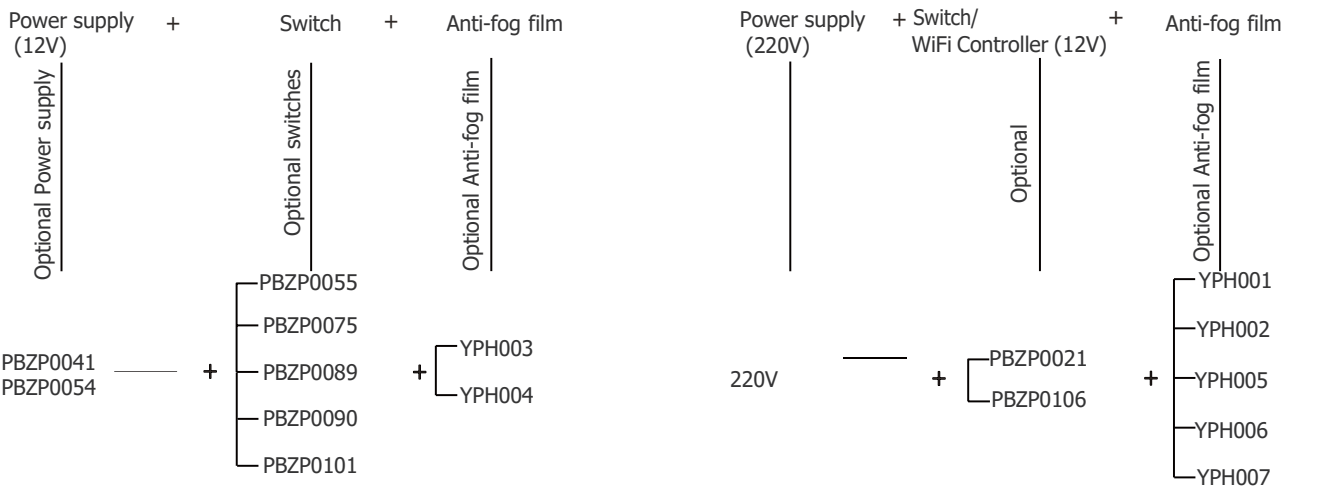
Hardware match figure 1 (power supply & switch & anti-fog film) Hardware match figure 2 (power supply & switch & anti-fog film)
