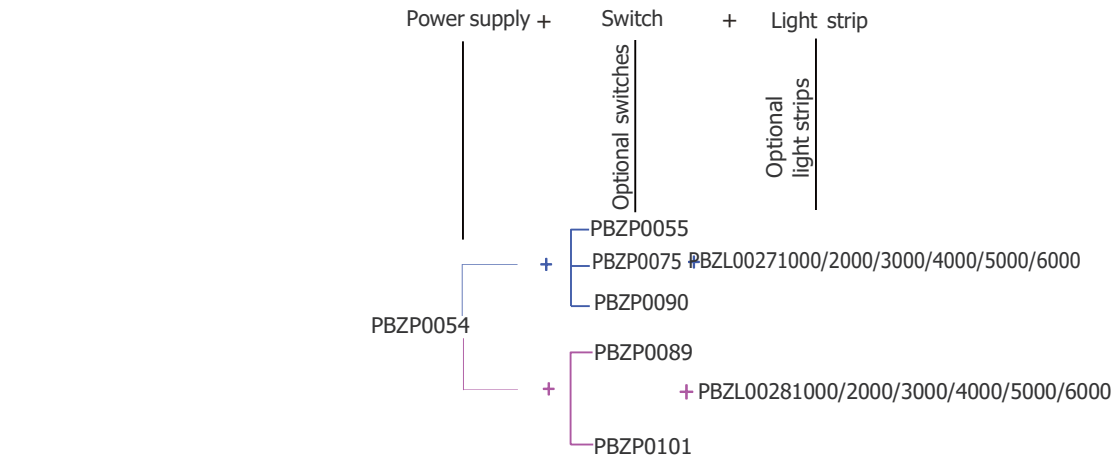
Hardware match figure 2 (power supply & switch & light strip)
